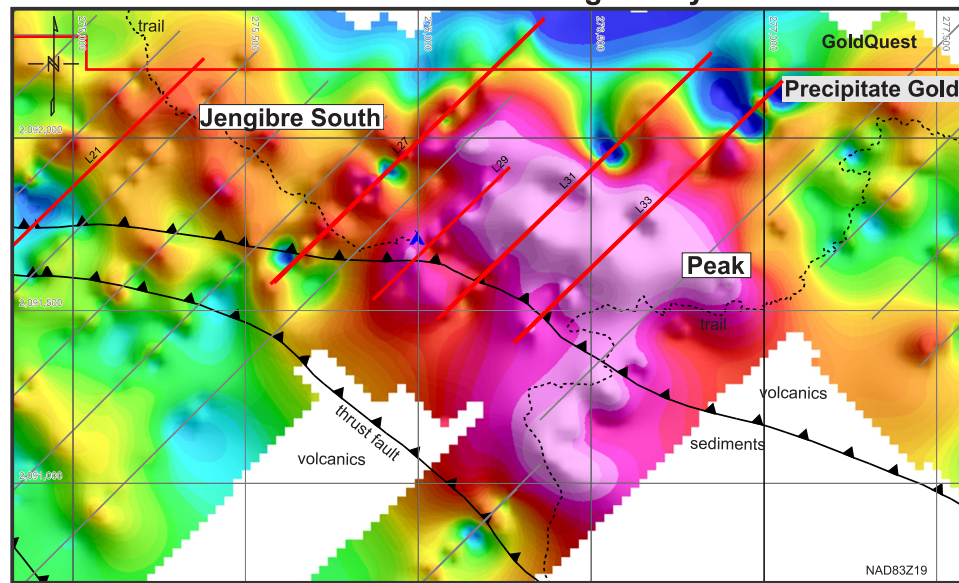
2026 Gradient IP Chargeability
